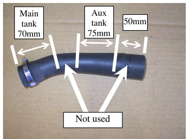
Photo 9: Prepare rubber filler hose
